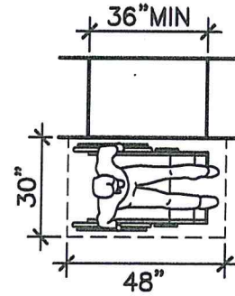
TRANSACTION COUNTER/ PARALLEL APPROACH
