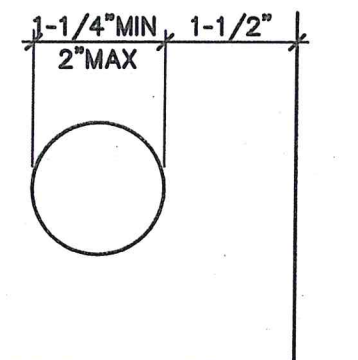
RAMP & STAIR HANDRAIL
