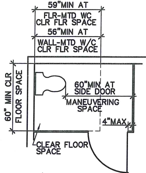
CLEARANCE AT WATER CLOSET IN COMPARTMENT WITH OUT-SWINGING SIDE-OPENING DOOR
