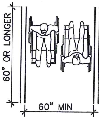
MINIMUM CLEAR WIDTH FOR TWO WHEELCHAIRS
