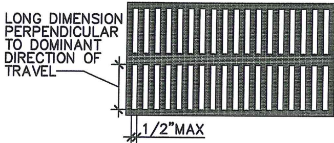
ELONGATED OPENINGS IN FLOOR OR GROUND SURFACES
