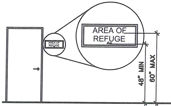
HEIGHT OF TACTILE CHARACTERS ABOVE FINISHED FLOOR OR GROUND
