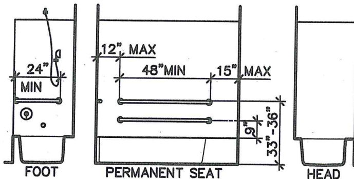
BATHTUBS WITH PERMANENT SEATS
