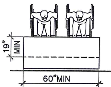
MINIMUM CLEARANCES FOR BAR SEATING
