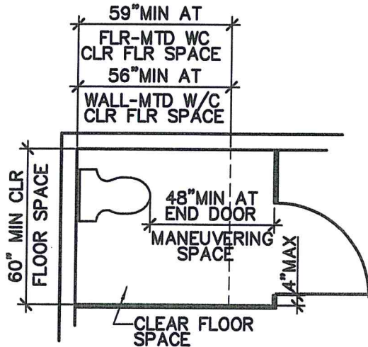
CLEARANCE AT WATER CLOSET IN COMPARTMENT WITH OUT-SWINGING END-OPENING DOOR
