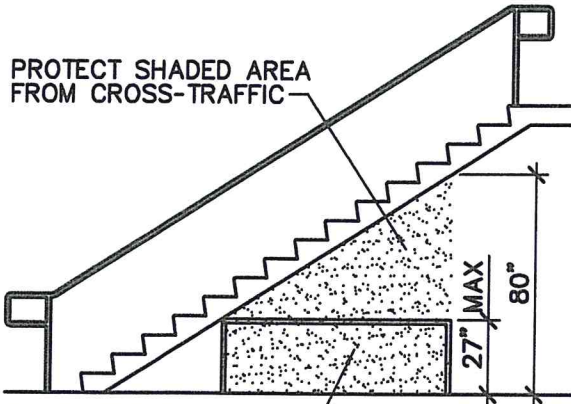
CANE DETECTION AREA OVERHEAD HAZARDS
