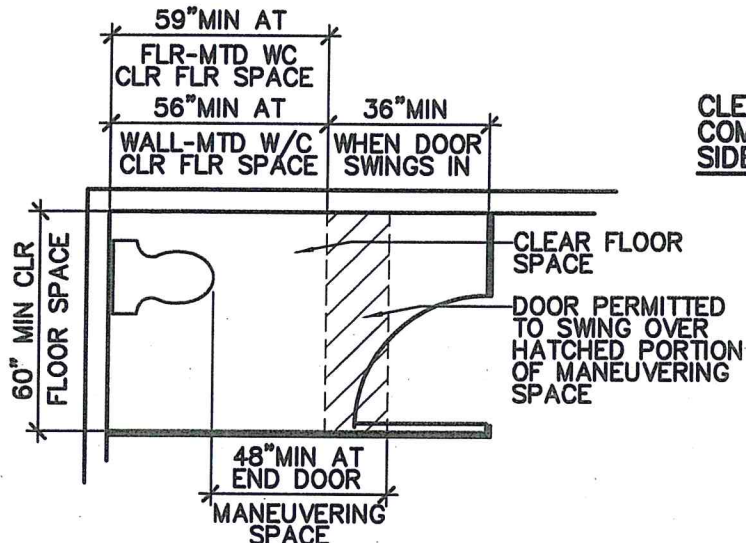
CLEARANCE AT WATER CLOSET IN COMPARTMENT WITH IN-SWINGING END-OPENING DOOR
