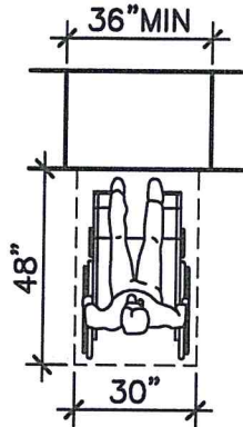
TRANSACTION COUNTER/ FORWARD APPROACH
