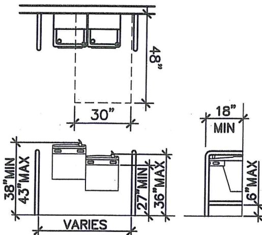
WING WALL DRINKING FOUNTAIN
