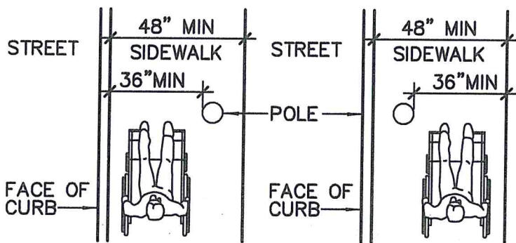
MINIMUM CLEAR WIDTH SIDEWALK OBSTRUCTIONS
