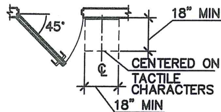
LOCATION OF TACTILE SIGNS AT DOORS
