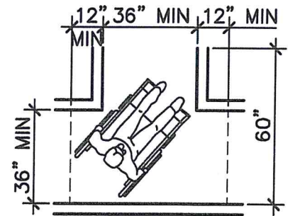
T-SHAPED SPACE FOR 180° TURNS
