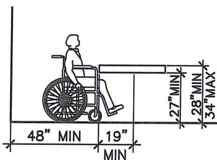
MINIMUM CLEARANCES FOR BAR SEATING
