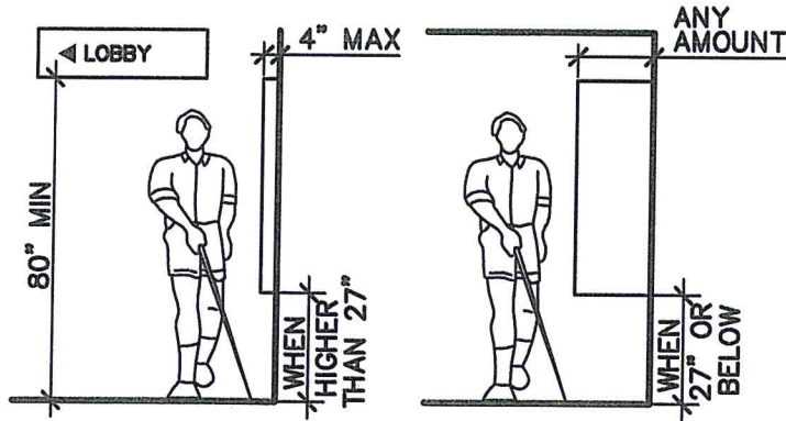
LIMITS OF PROTRUDING OBJECTS
