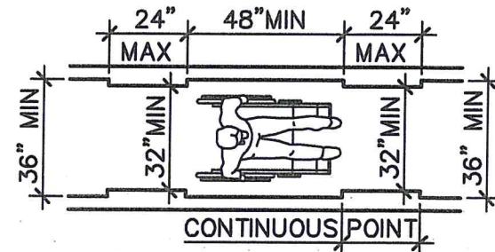
MINIMUM CLEAR WIDTH FOR SINGLE WHEELCHAIR
