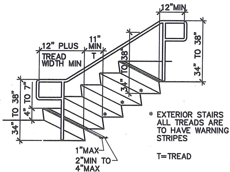
WARNING STRIPING & HANDRAIL EXTENSIONS
