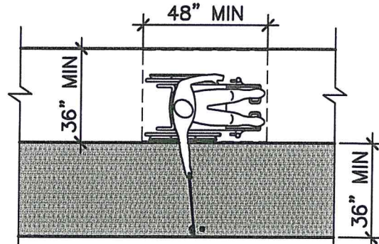
RUNNING SLOPE OF CLEAR FLOOR OR GROUND SPACE NOT STEEPER THAN 1:20 (5%) GOLF CLUB REACH RANGE AREA
