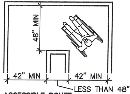
ACCESSIBLE ROUTE TURNS AROUND AN OBSTRUCTION *
