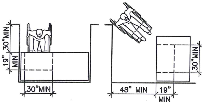
MINIMUM CLEARANCES FOR SEATING AND TABLES
