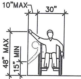
HIGH & LOW SIDE REACH LIMITS
