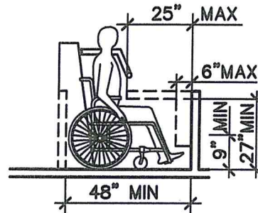
PROTRUSIONS IN WHEELCHAIR SPACES IN AMUSEMENT RIDES
