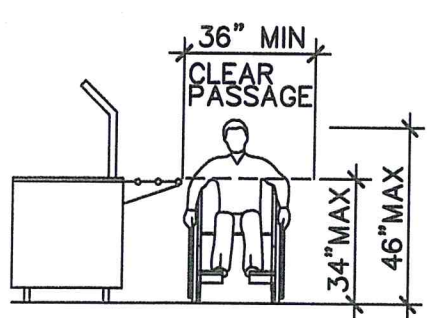
FOOD SERVICE LINES
