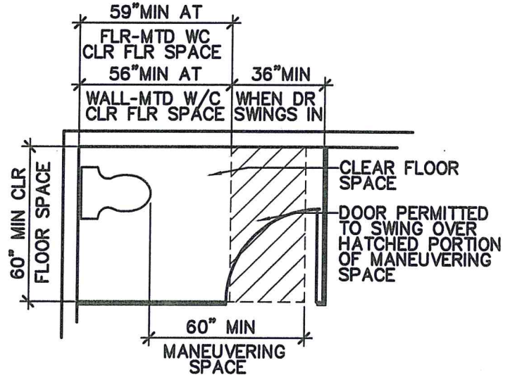
CLEARANCE AT WATER CLOSET IN COMPARTMENT WITH IN-SWINGING SIDE-OPENING DOOR
