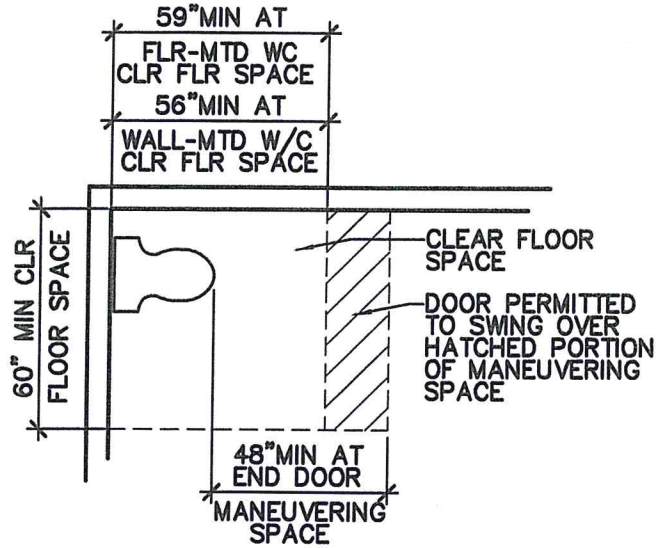
CLEARANCE AT WATER CLOSET
