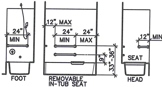
BATHTUBS WITH REMOVABLE IN-TUB SEATS
