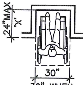
36" WHEN 'X' > 24" FORWARD APPROACH
