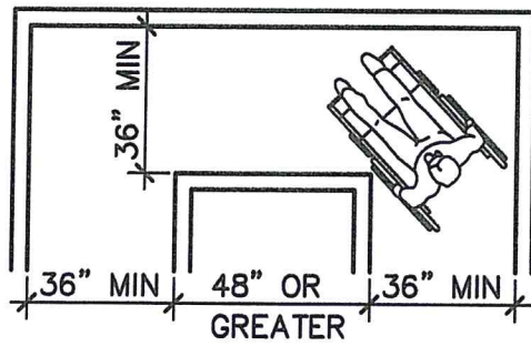
ACCESSIBLE ROUTE FOR 90° TURNS *
